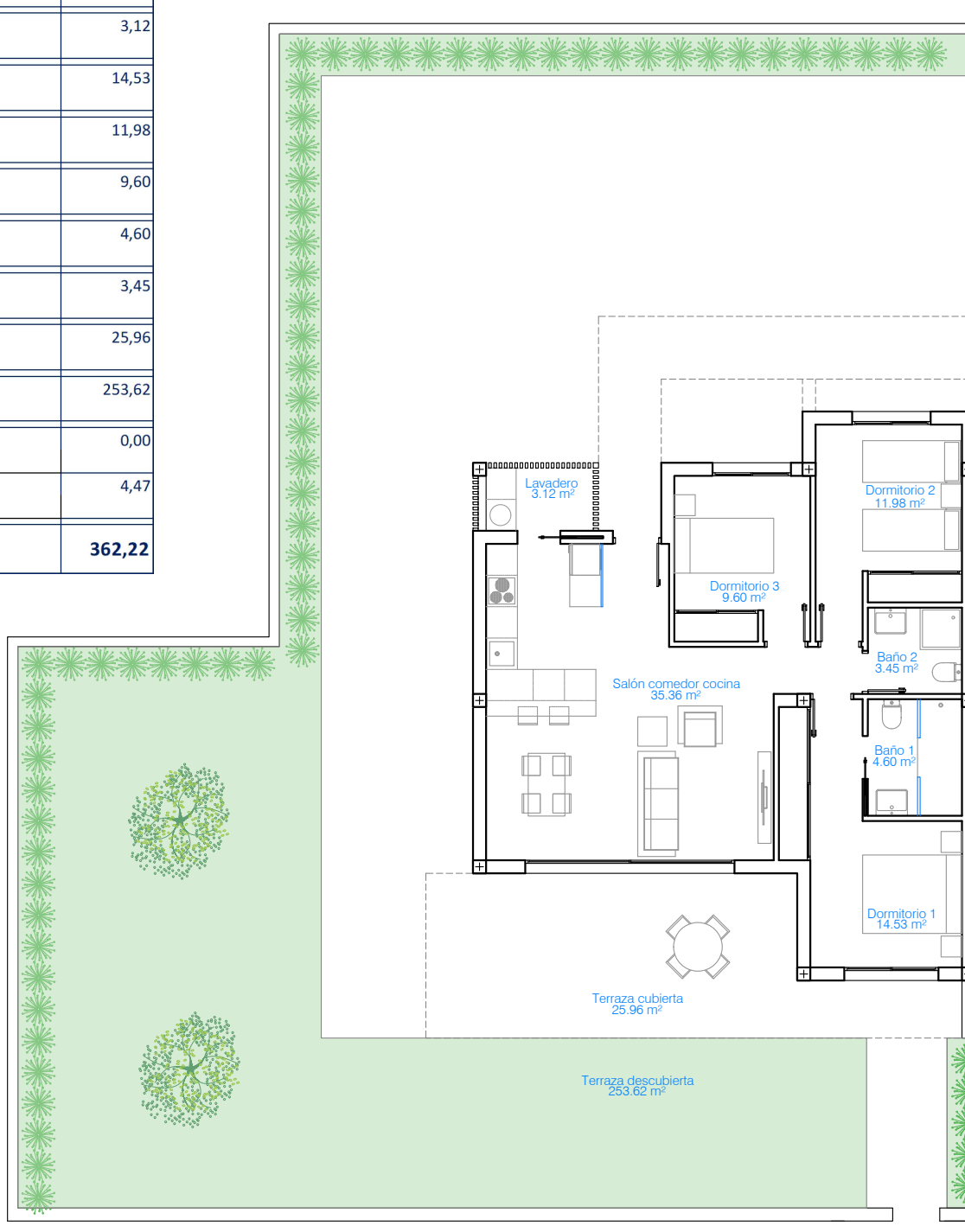
Ground Floor/ Planta Baja (E:1/125)
