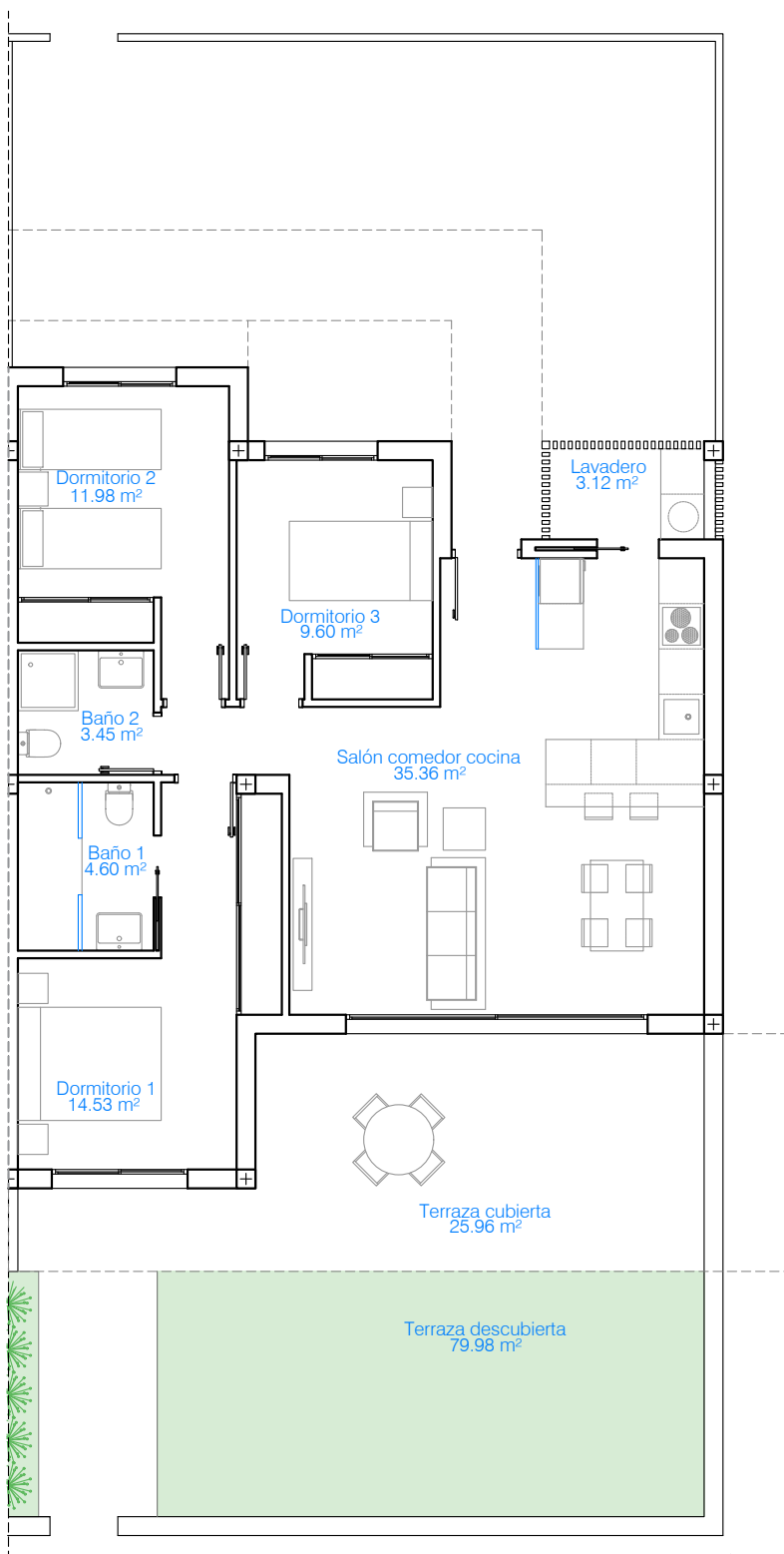
Ground Floor/ Planta Baja (E:1/100)
